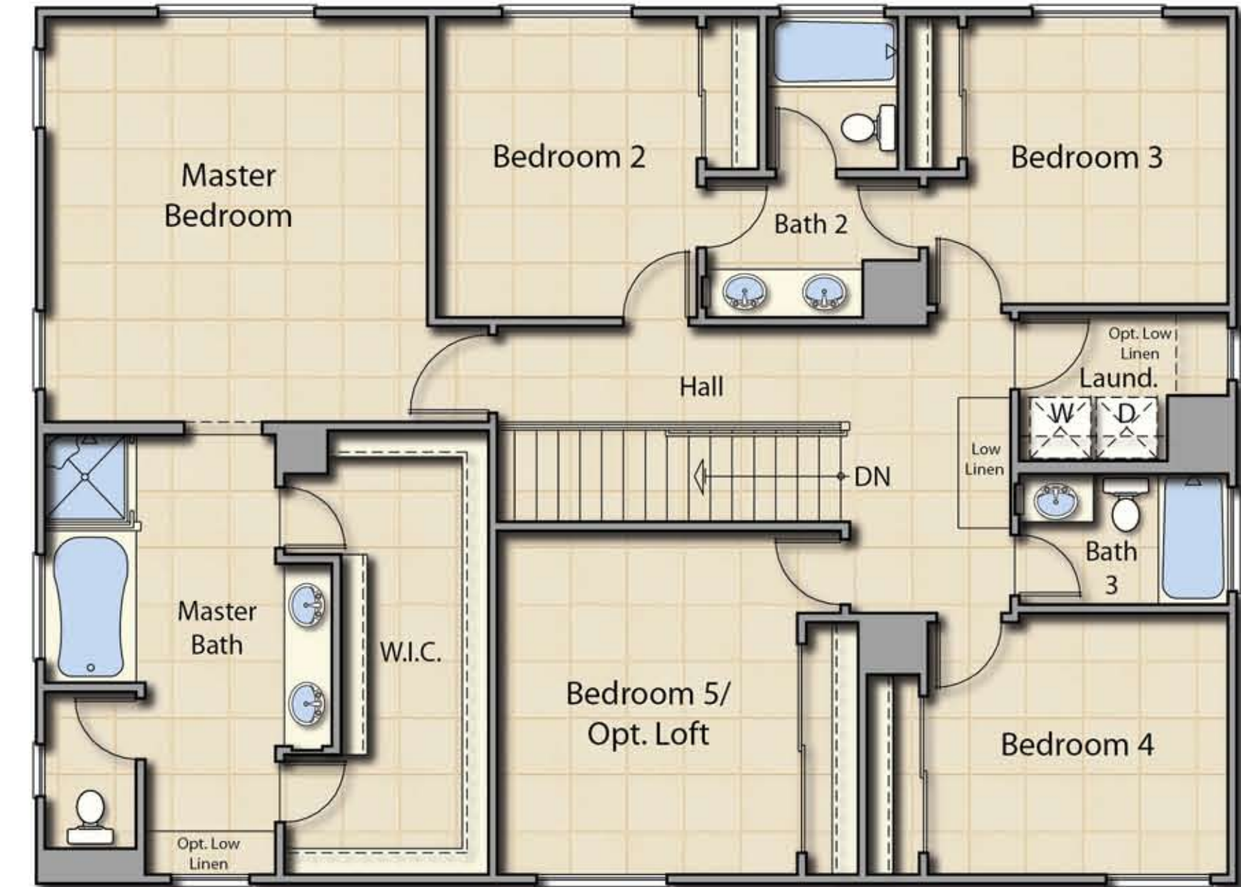
SECOND FLOOR
